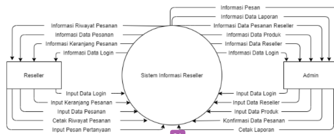
Gambar 4. DFD level 0
