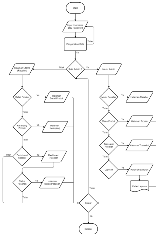
Gambar 3. Flowchart system
