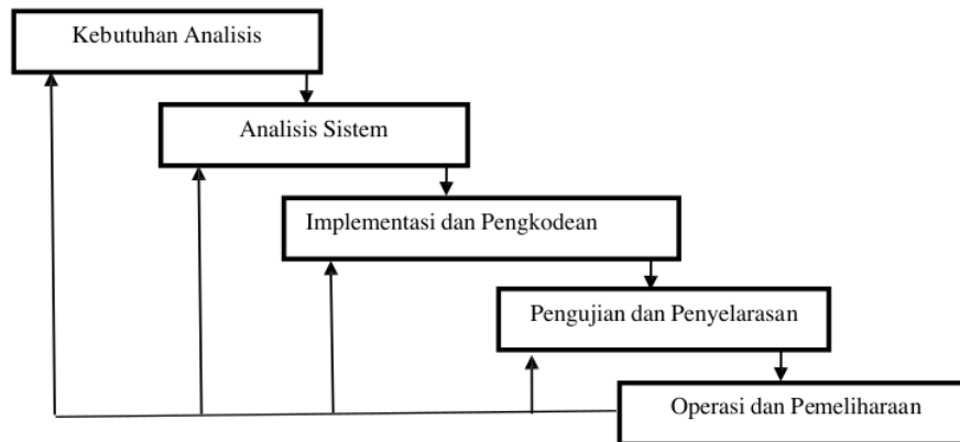
Gambar 1. Metode Waterfall
