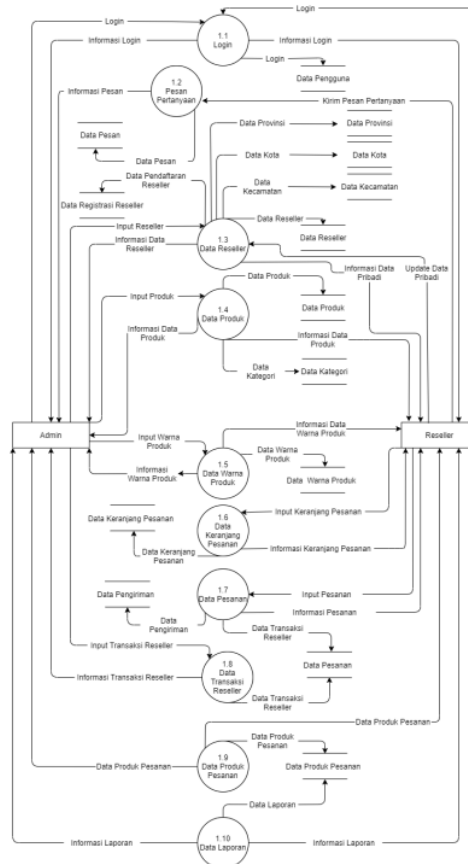
Gambar 5. DFD level 1
